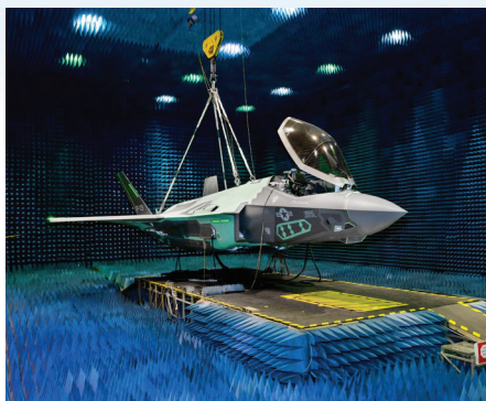
Anechoic chamber testing of the F-35A CTOL variant.
